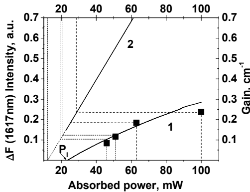
Fig. 6. Curves 1 and 2 (left scale) show the increase of the 1617 nm fluorescence intensities at powers above the inversion threshold. 1-ΔF from experimental data measured without output coupler, 2-ΔF i calculated from the extrapolation of the linear portion of dependence F=f(P p ) at low excitation level. Solid squares display the threshold gain (right scale) at different output couplers.
