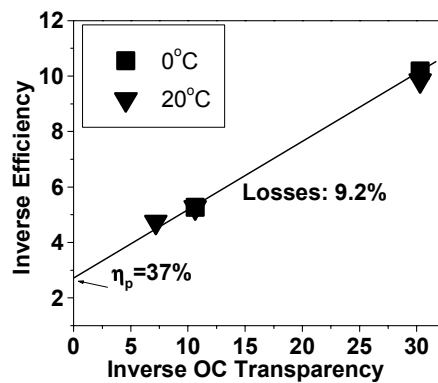
Fig. 4. Inverse absorbed photon conversion efficiency ( 1/\eta ) vs. inverse output coupler transmission at T=0°C and T=20°C.
