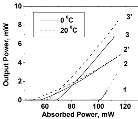
Fig. 3. Output power as a function of absorbed power for 1470-nm pumped Er 3+ :YAG DPSSL with different output couplers: 1 - T=3.3%, 2 - T=9.4%, 3 - T=13.9%. Curves 1, 2 and 3 were measured at rod temperature 0°C and dashed curves 2', and 3' at 20°C.
