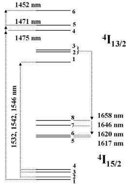
Fig. 1. Er 3+ :YAG absorptive and radiative transitions in the 1.45-1.66 μm spectral range.
