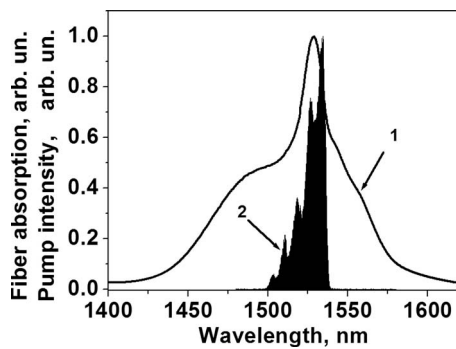
FIG. 2. Combined spectrum of the six 1530 nm fiber-coupled laser diode modules at 27 W of output power (curve 2) overlaid with the Er60-20/125DC fiber absorption (curve 1).
